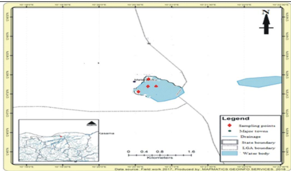
Fig. 1. Matara-Uku wetland along Hadejia-Nguru wetlands
