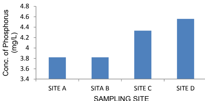
Fig. 3. Mean concentration of phosphorus
