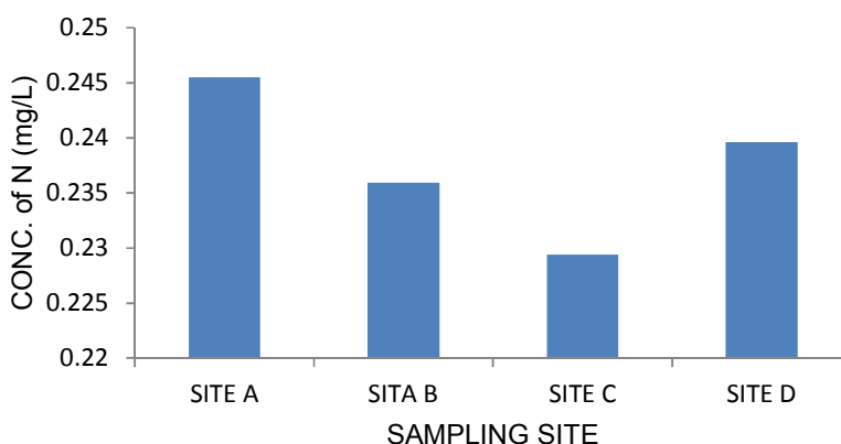
Fig. 4. Mean concentration of nitrogen
