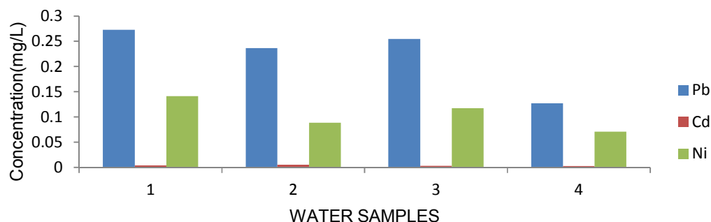
Fig. 5. Mean concentration of heavy metals
