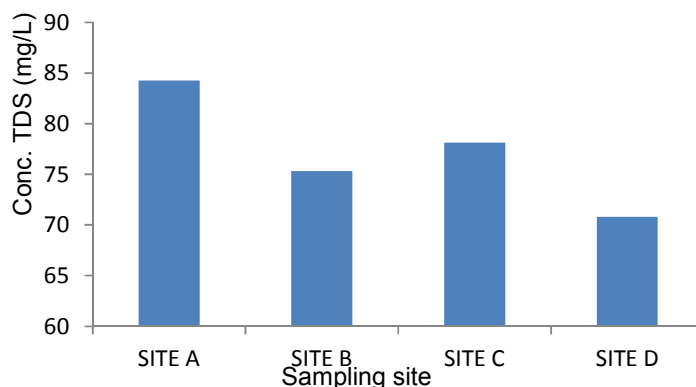
Fig. 2. Mean concentration of total dissolve solid
